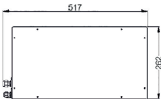
Front view evaporator unit :
